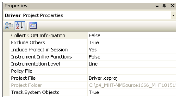
Figure 6-6. Project Properties
