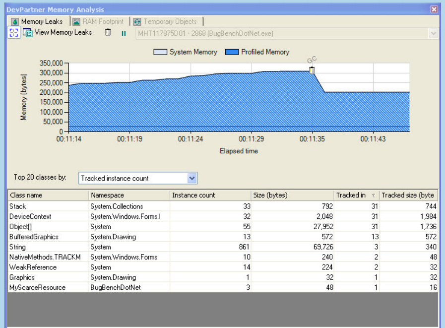
Figure 5-3. Session Control Window After Garbage Collection
