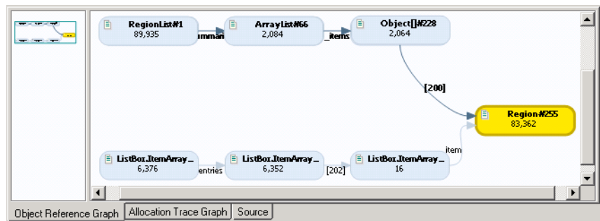
Figure 5-21. The Object Reference Graph Shows Why an Object is Still in Memory
