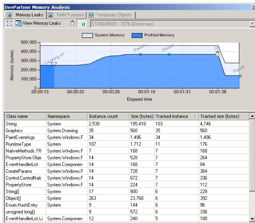
Figure 5-12. DevPartner Memory Analysis Session Control Window
