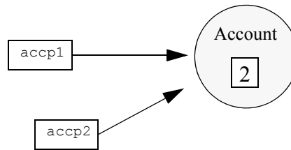
Figure 9: Reference for Account proxy is incremented to 2.
