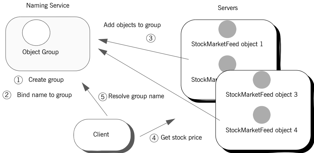
Figure 31: Architecture of the stock market example
