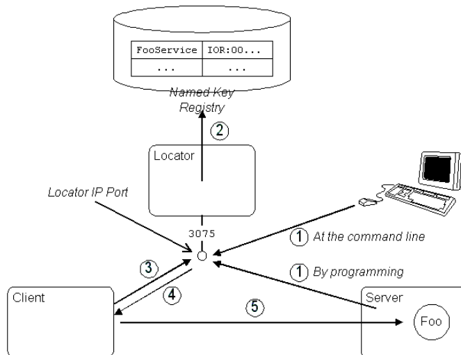
Figure 55: Using corbaloc with the Locator-Based Named Key Registry
