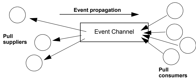
Figure 40: Pull Model suppliers and consumers communicating through an event channel
