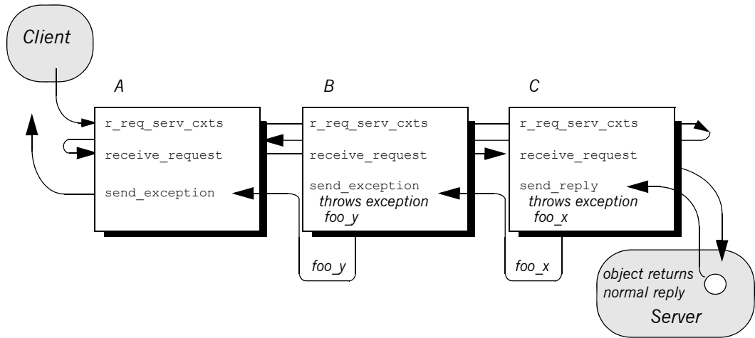
Figure 51: Server interceptors can change the reply type.
