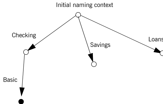
Figure 25: Binding an object reference to a naming context
