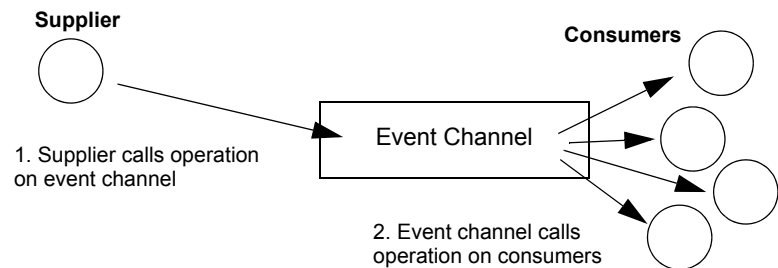
Figure 38: Event propagation in a CORBA system
