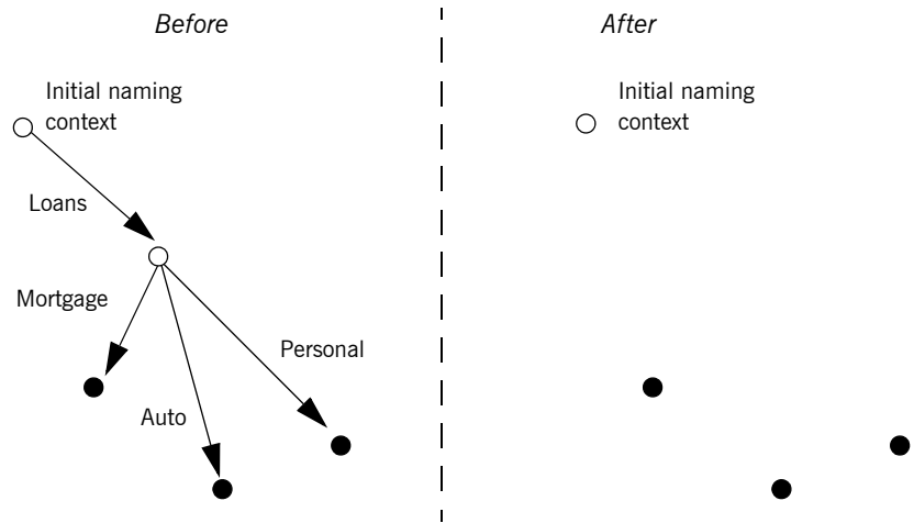
Figure 26: Destroying a naming context and removing related bindings
