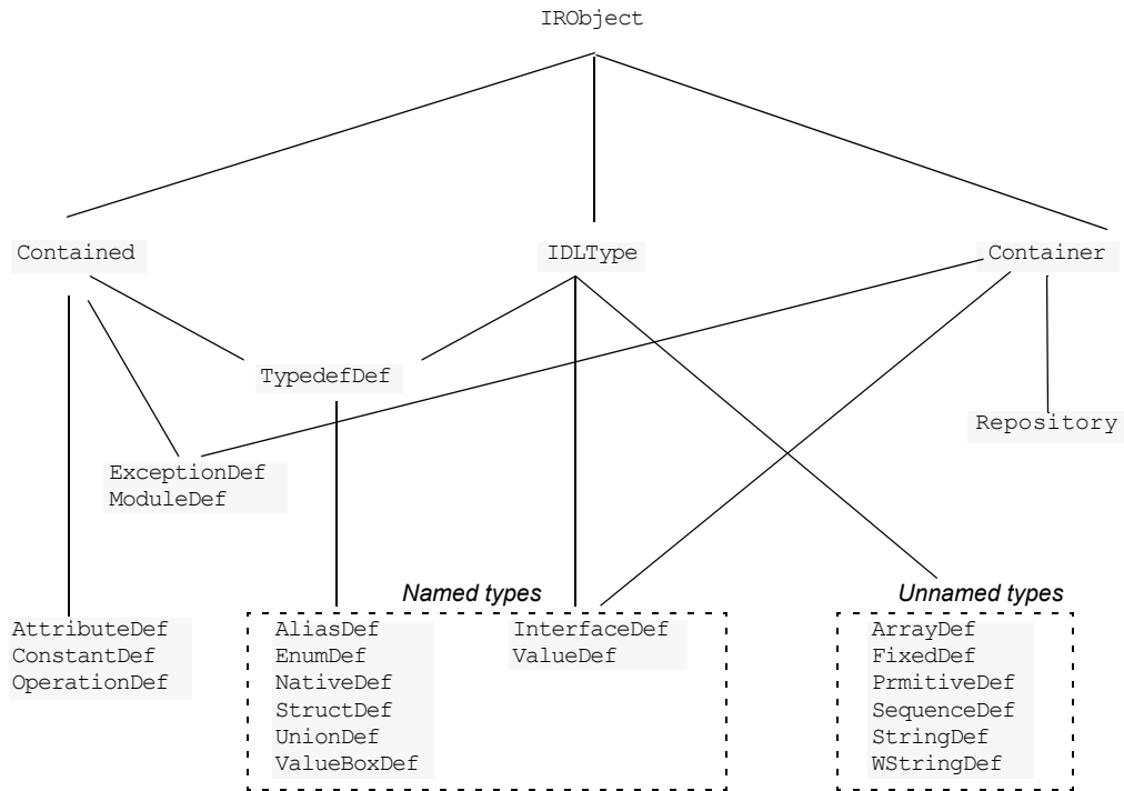
Figure 21: Hierarchy of interface repository objects
