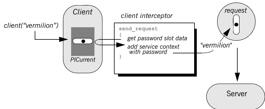
Figure 44: PICurrent facilitates transfer of thread context data to a request or reply.
