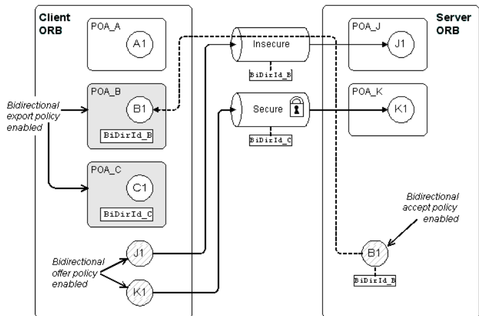
Figure 53: Advanced Bidirectional GIOP Scenario
