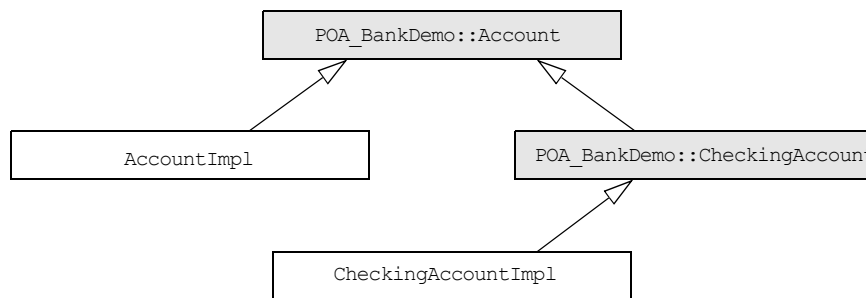
Figure 13: A servant class can implement operations of all base skeleton classes.
