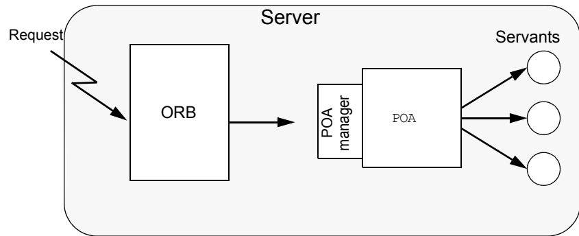
Figure 11: The server-side ORB conveys client requests to the POA via its manager, and the POA dispatches the request to the appropriate servant.
