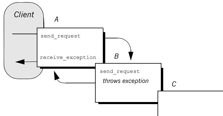
Figure 47: send_request throws an exception in a client-side interceptor
