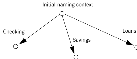
Figure 24: Savings and Loans naming contexts bound to initial naming context
