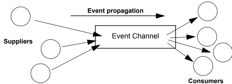
Figure 37: Suppliers and consumers communicating through an event channel
