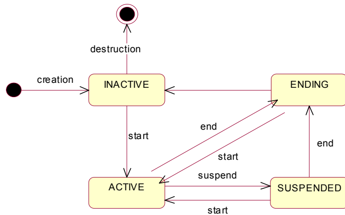
Figure 33: Transactional session states
