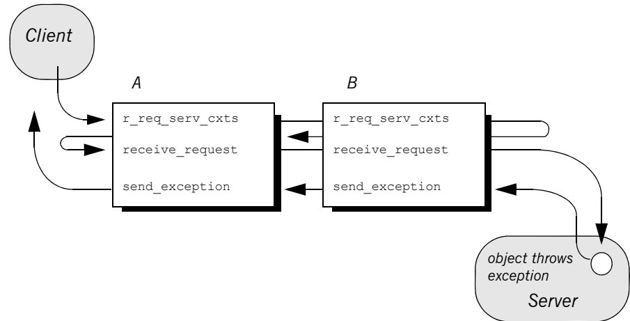
Figure 49: Server interceptors receive request and send exception thrown by target object.
