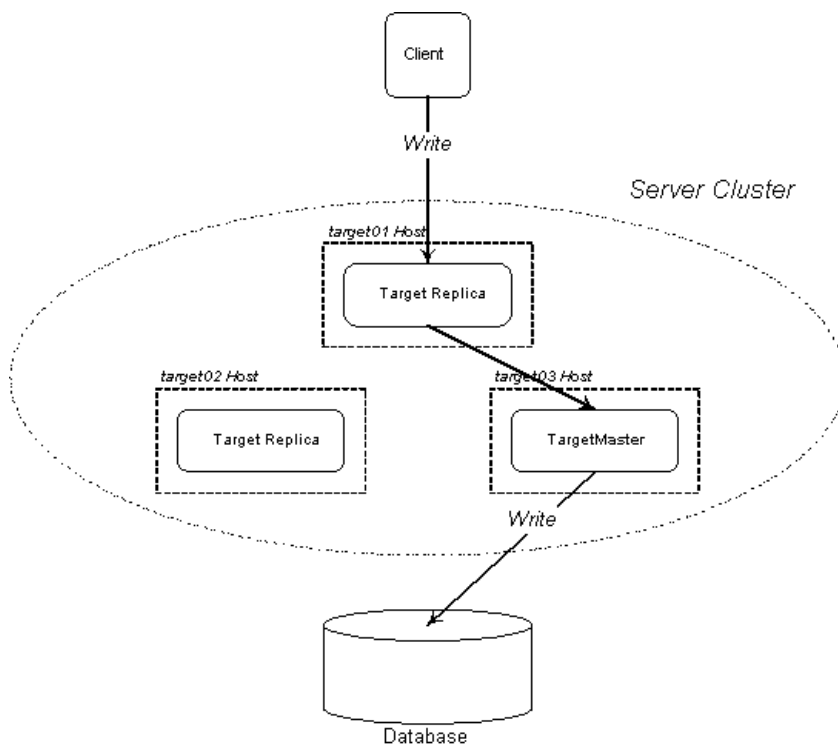
Figure 36: Delegation Required for Write Operation
