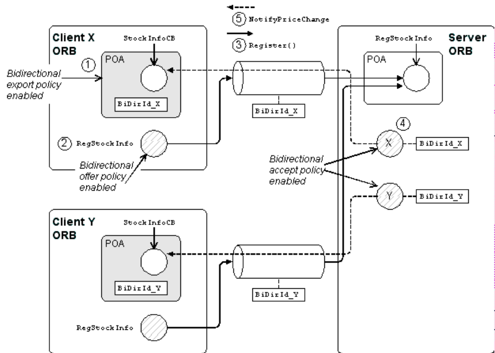
Figure 52: Basic Bidirectional GIOP Scenario—Stock Feed
