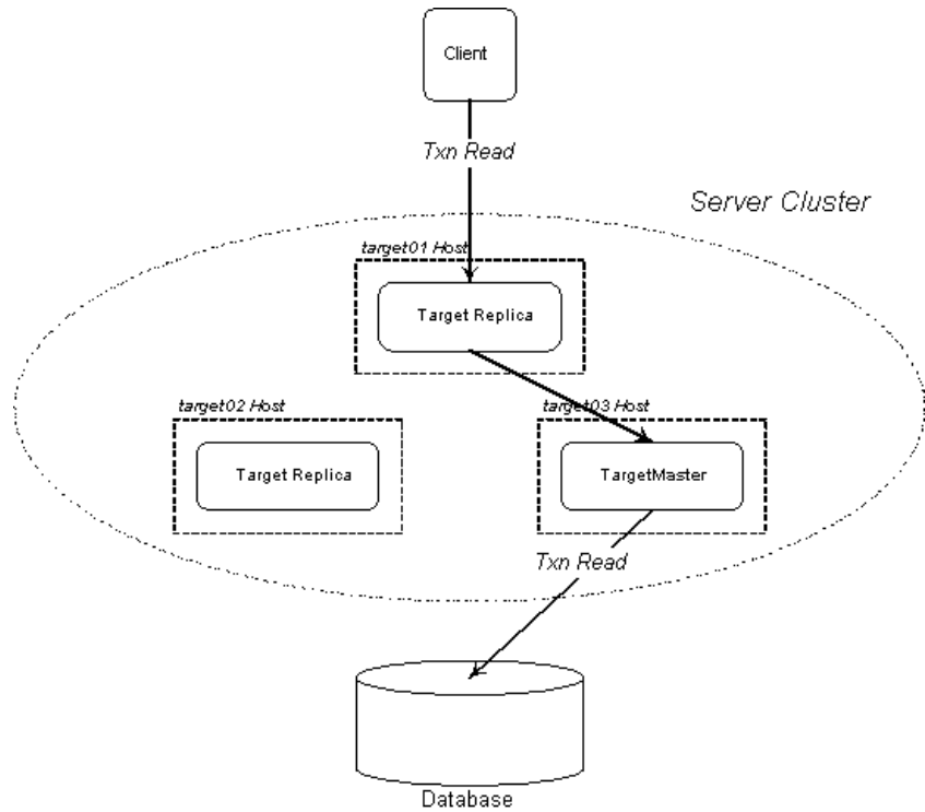
Figure 35: Delegation Required for Transactional Read Operation
