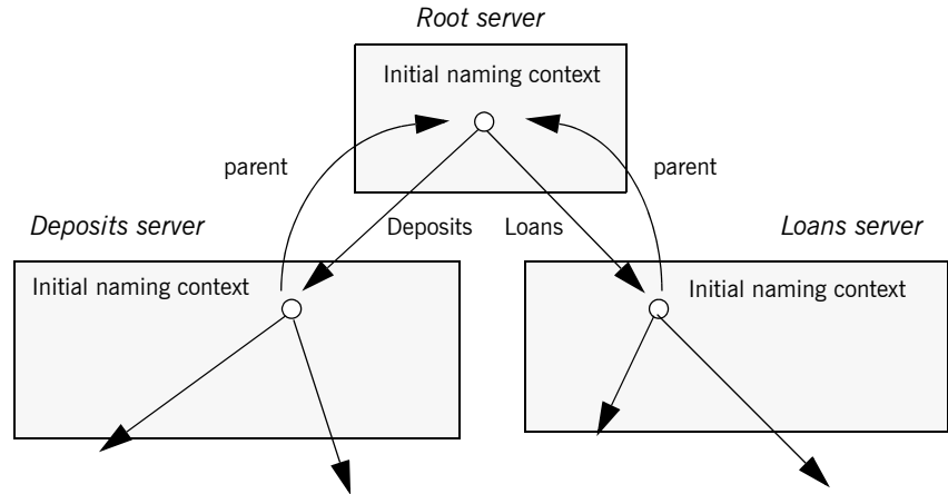
Figure 29: The root server's initial naming context is bound to the initial naming contexts of other servers, allowing clients to locate the root naming context.
