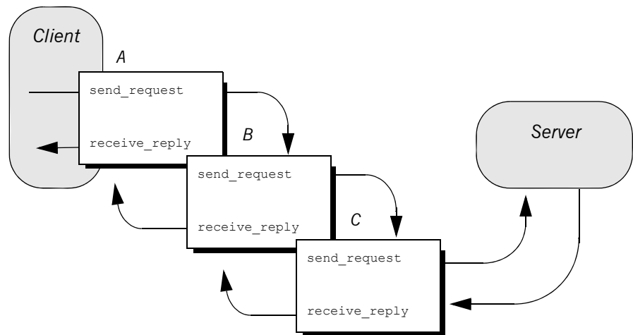
Figure 45: Client interceptors process a normal reply.
