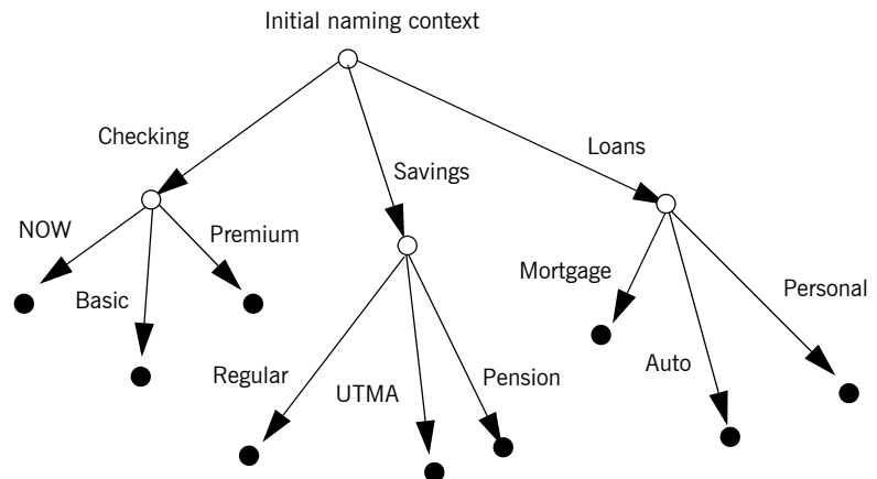
Figure 22: A naming graph is a hierarchy of naming contexts
