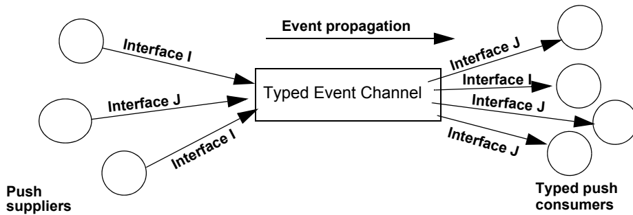
Figure 42: Push consumers pushing typed events to typed push consumers
