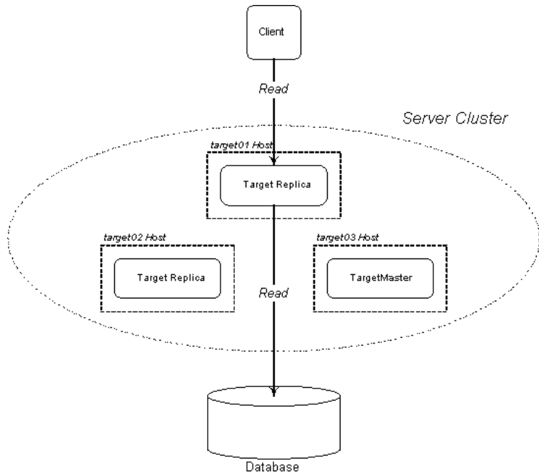
Figure 34: No Delegation Required for Ordinary Read Operation
