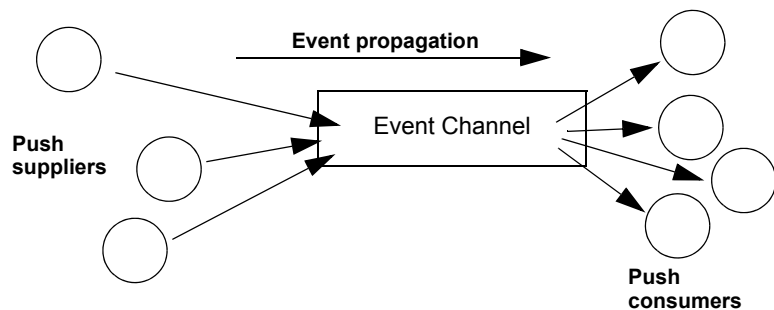
Figure 39: Push model of event transfer
