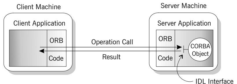
Figure 5: Client makes a single operation call on a server
