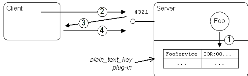
Figure 56: Using corbaloc with the plain_text_key Plug-In
