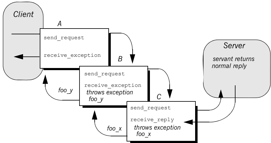
Figure 48: Client interceptors can change the nature of the reply.
