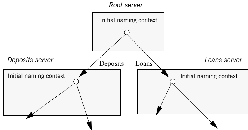
Figure 28: Multiple naming graphs are linked by binding initial naming contexts of several servers to a root server.
