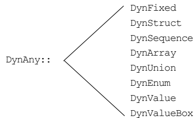
Figure 20: Interfaces that derive from the DynAny interface
