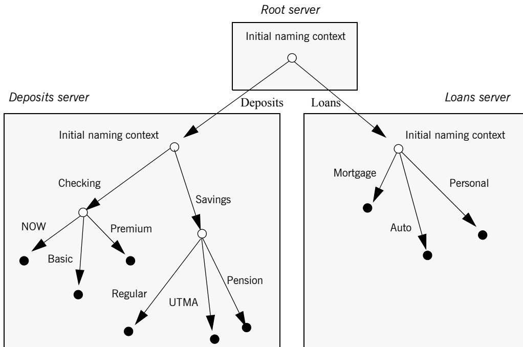
Figure 27: A naming graph that spans multiple servers
