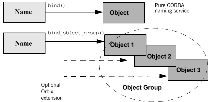
Figure 30: Associating a name with an object group
