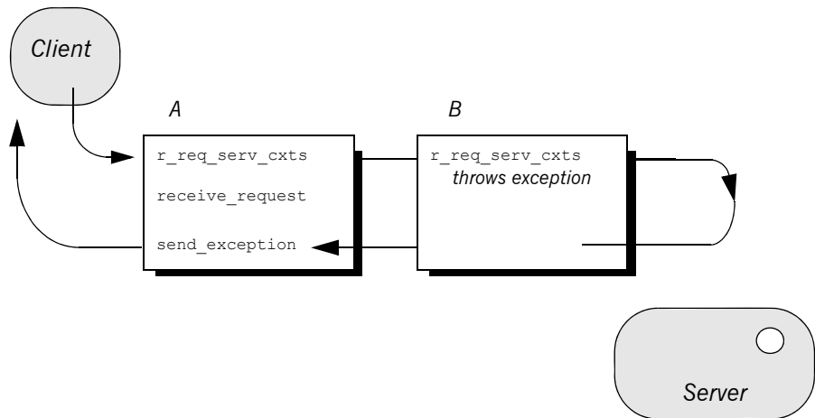
Figure 50: receive_request_service_contexts throws an exception and interception flow is aborted.
