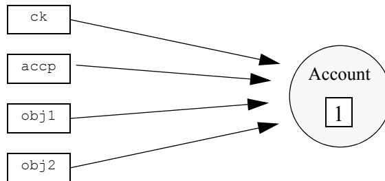
Figure 10: Multiple _ptr references to a proxy object can leave the reference count unchanged.
