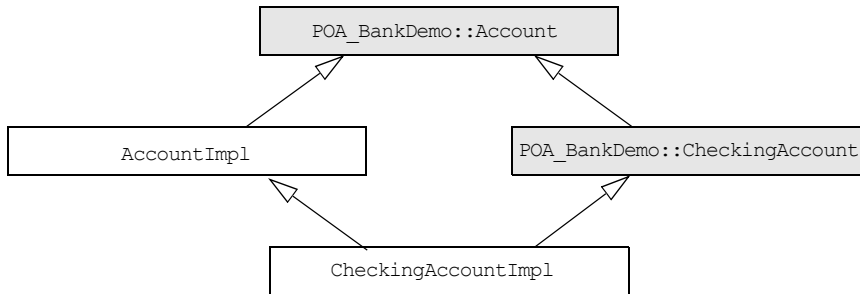
Figure 12: A servant class can inherit base class implementations.
