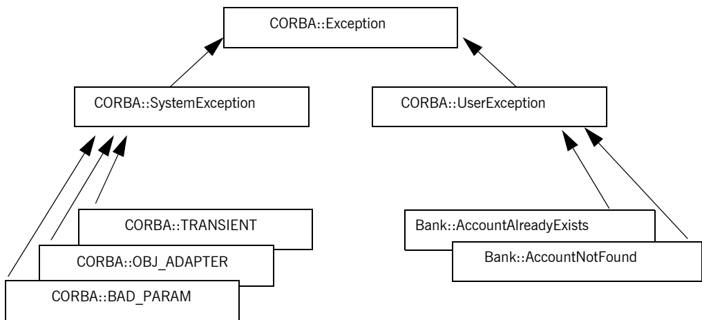
Figure 19: The C++ mapping arranges exceptions into a hierarchy
