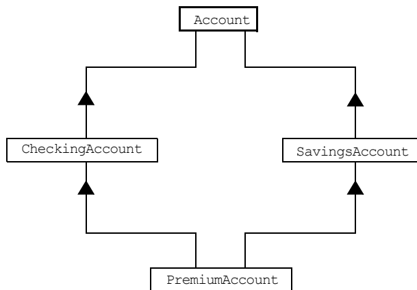
Figure 7: Multiple inheritance of IDL interfaces
