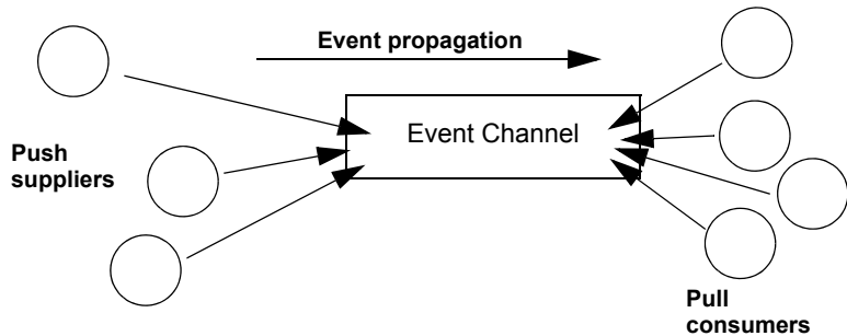
Figure 41: Push suppliers and pull consumers communicating through an event channel
