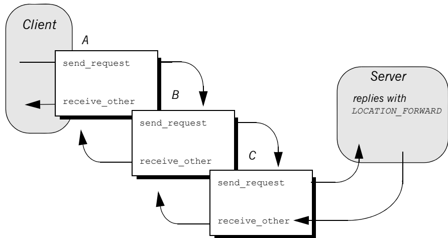
Figure 46: Client interceptors process a LOCATION_FORWARD reply.
