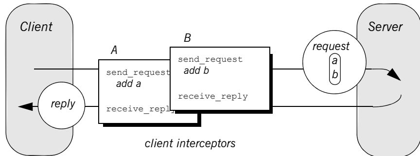
Figure 43: Client interceptors allow services to access outgoing requests and incoming replies.
