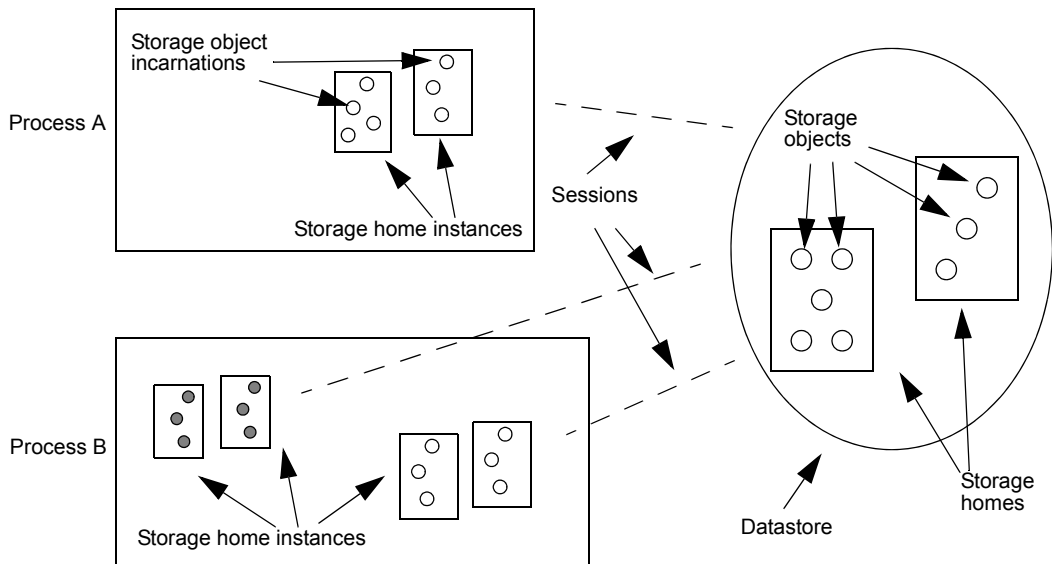
Figure 32: A server process uses sessions to establish a logical connection with a datastore and its contents
