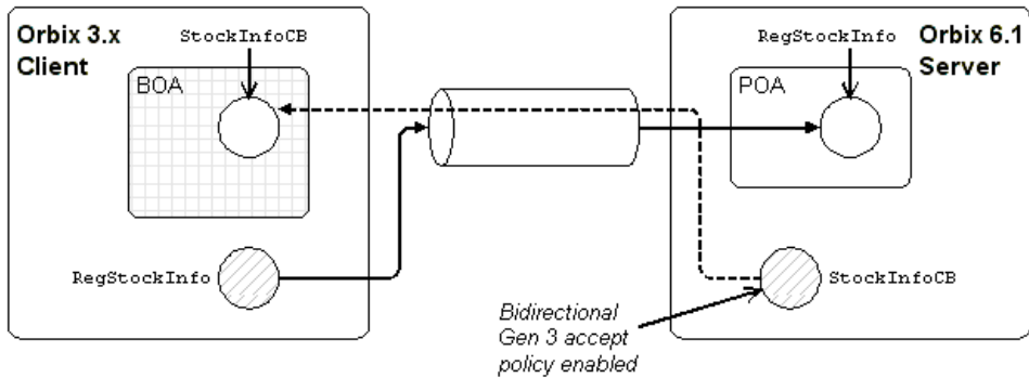
Figure 54: Orbix 3 Client Receiving a Callback from an Orbix 6.1 Server
