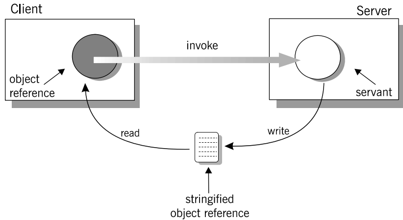
Figure 6: Simple strategy for passing object references to clients
