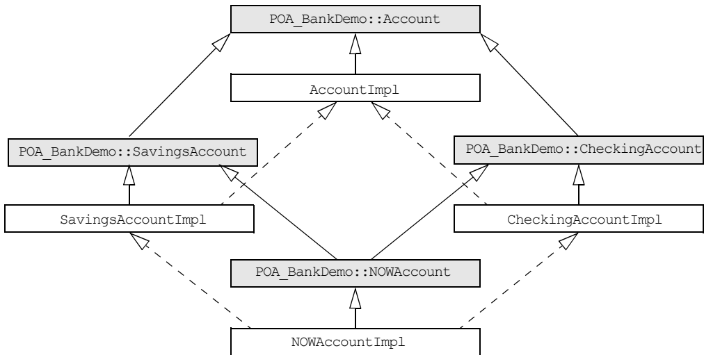
Figure 14: Inheritance options among servant and base skeleton classes.
