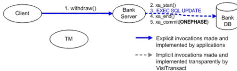
Figure 25 Server-initiated transaction
